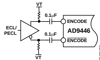
Figure 60. Differential ECL for Encode
