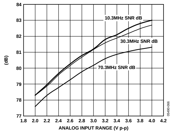
Figure 53. AD9446-80/SNR vs. Analog Input Range, 80 MSPS
