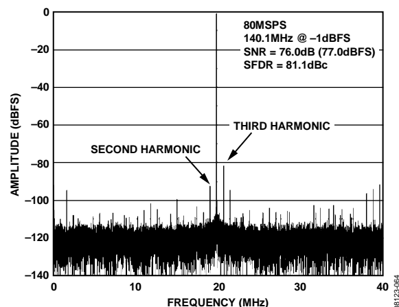
Figure 10. AD9268-80 Single-Tone FFT with f_{IN} = 140.1 MHz
