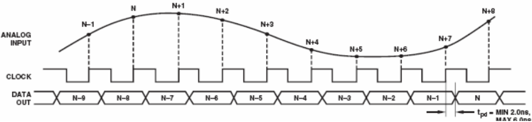
Figure 2. Timing Diagram
