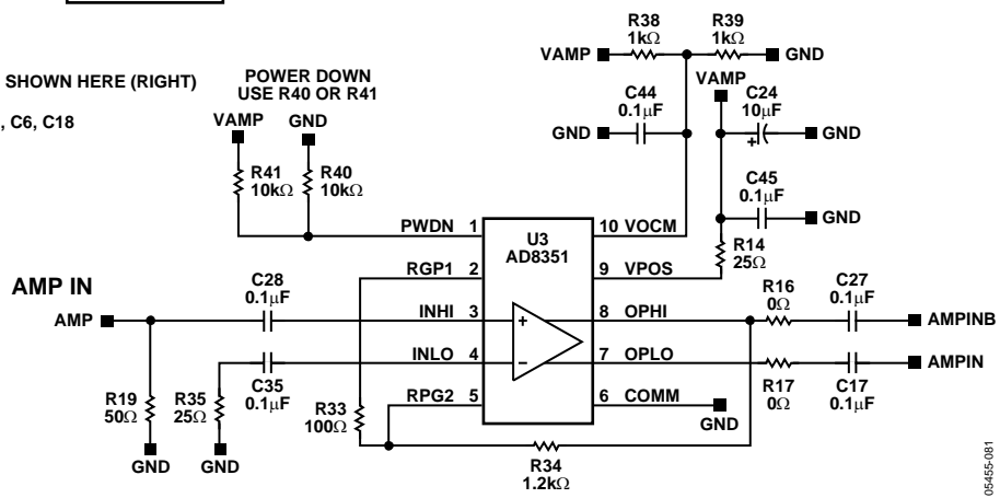
Figure 49. LFCSP Evaluation Board Schematic, Digital Path
