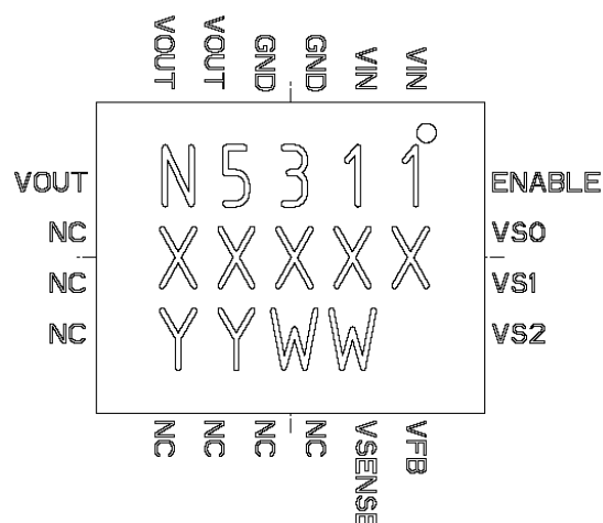
Figure 2. Pin description, top view.
