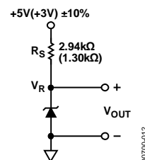
Figure 12. Typical Connection Diagram
