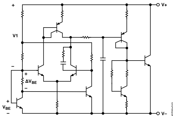
Figure 10. Schematic Diagram
