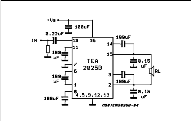
Figure 3. Bridge application
