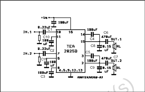
Figure 4. Stereo application
