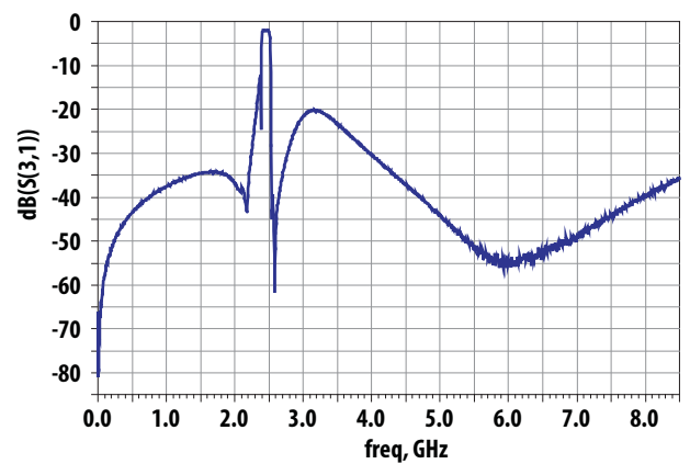
Figure 6. RX Path 0 – 8.5 GHz Frequency Response
