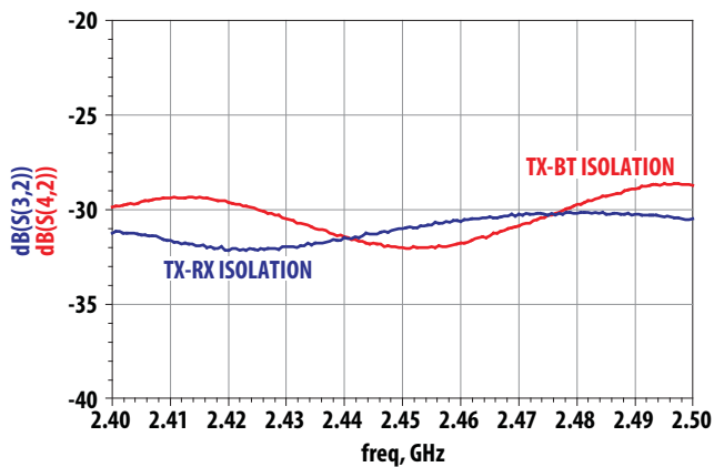
Figure 11. TX-RX and TX –BT Isolation in 2.4 – 2.5 GHz Band
