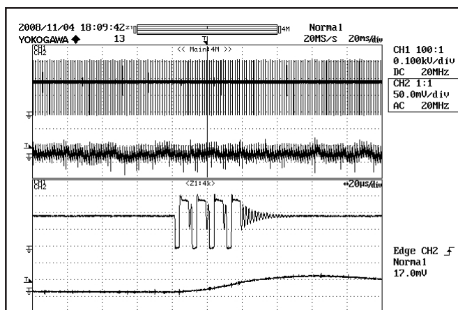
Top Trace: Drain Waveform (200 V/div) Bottom Trace: Output Ripple Voltage (50 mV/div)
