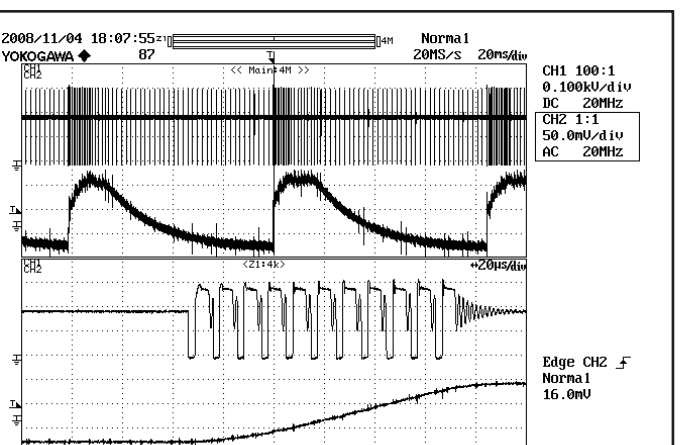
Split Screen with Bottom Screen Zoom Top Trace: Drain Waveform (200 V/div) Bottom Trace: Output Ripple Voltage (50 mV/div)
