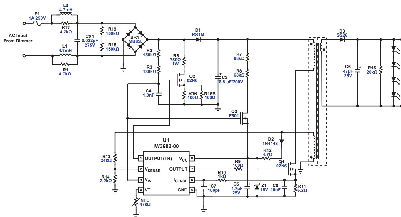
Figure 11.1 : iW3602-00 Typical Application Schematic
