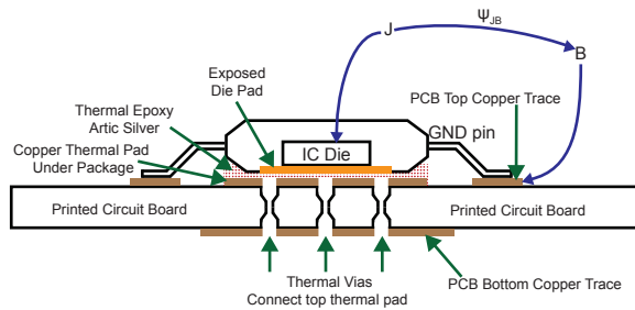
Figure 9.13 : Ways to Improve Thermal Resistance
