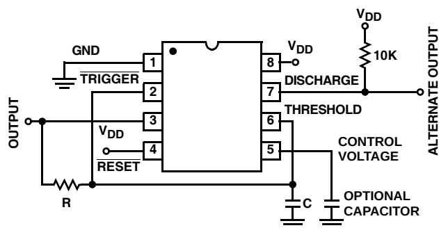
FIGURE 2A. ASTABLE OPERATION
