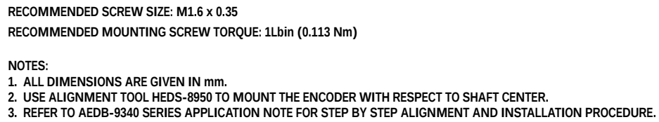
Figure 4b. 1000/2000 CPR encoder module mounting considerations
