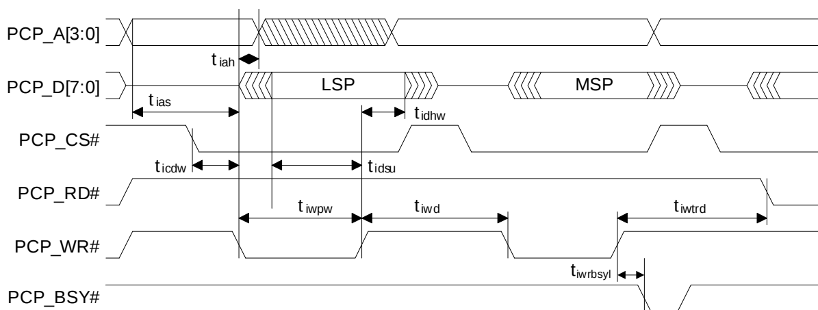
Figure 8. Parallel Control Port - Intel Slave Mode Write Cycle
