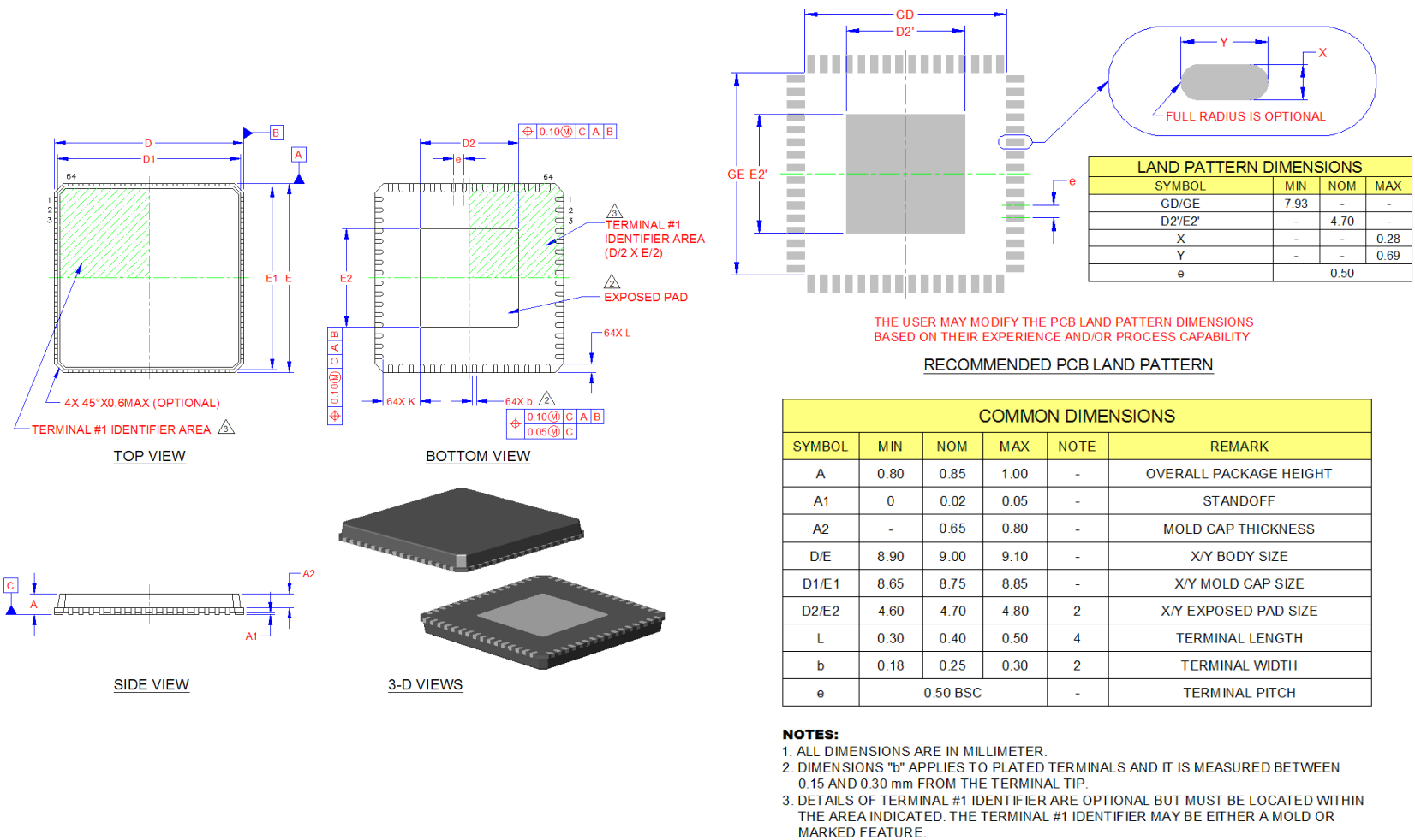
Figure 10.1 64-Pin QFN, 9x9mm Body, 0.5mm Pitch
