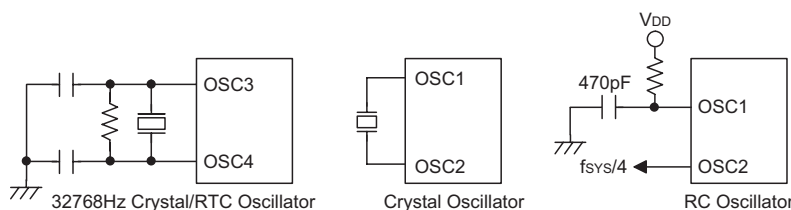
System Oscillator
