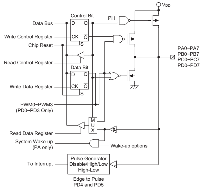
Input/Output Ports
