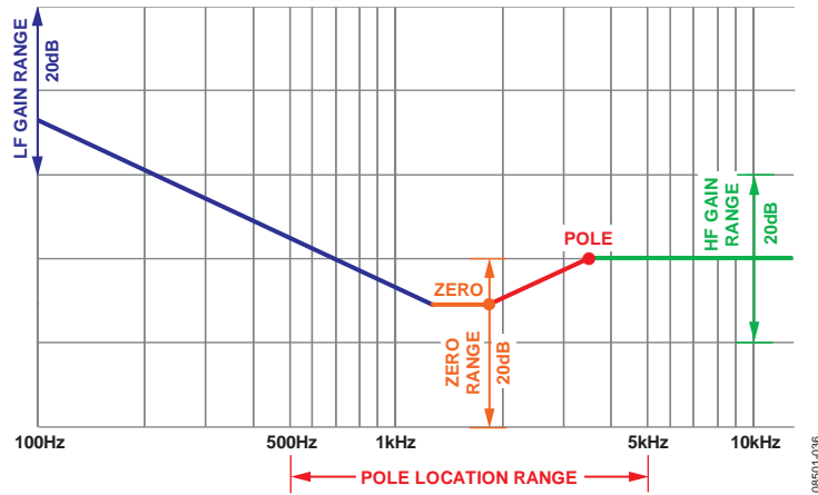
Figure 37. Digital Filter Programmability
