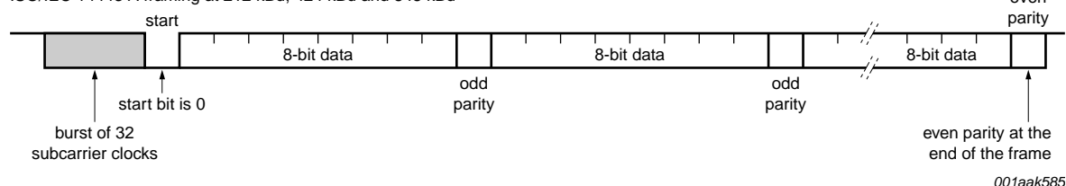
Fig 6. Data coding and framing according to ISO/IEC 14443 A
