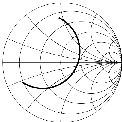
Figure 17. Input Impedance, 3 \mu A Bias.
