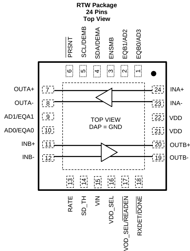
Pin Functions (1)(2)(3)(4)
