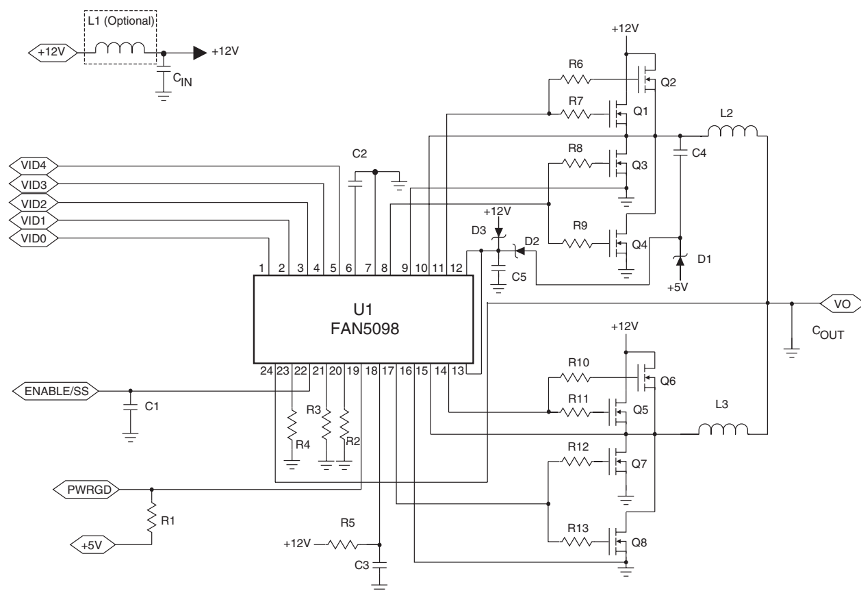
Figure 2. Application Circuit for 42A AMD Hammer Desktop Application
