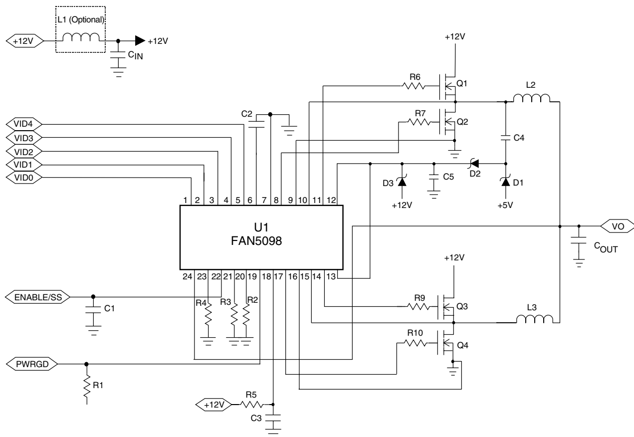
Figure 1. Application Circuit for 31A AMD Hammer Desktop Application (500 KHz each phase)
