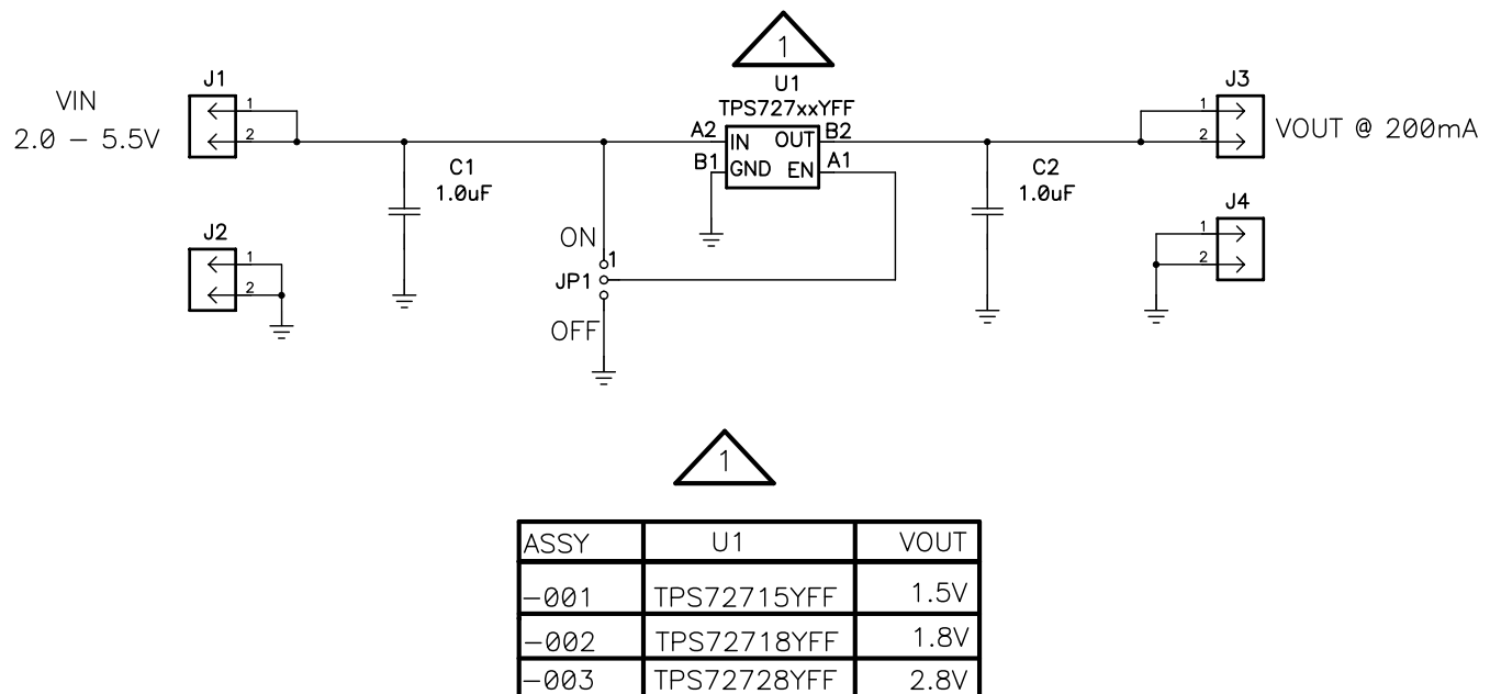
Figure 25. TPS727xxYFFEVM-407 Schematic
