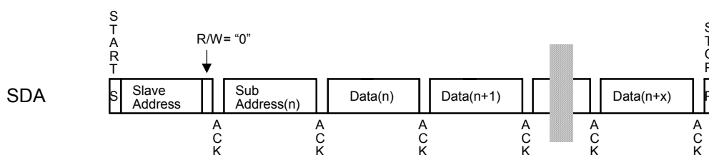
Figure 7. Data transfer sequence at the I 2 C-bus mode
