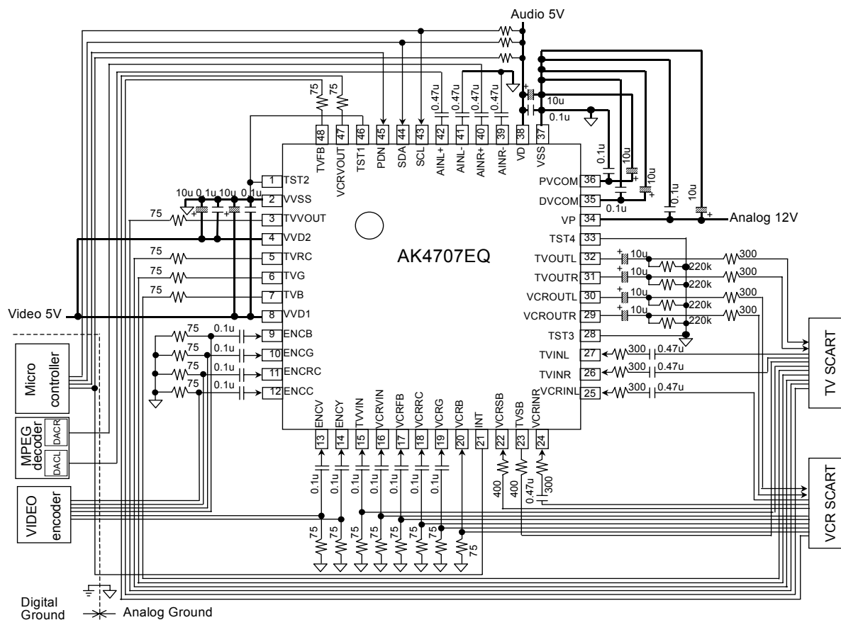
Figure 17. Typical Connection Diagram (Single-ended Input )
