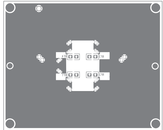
Figure 14. CEB018 Bottom View
