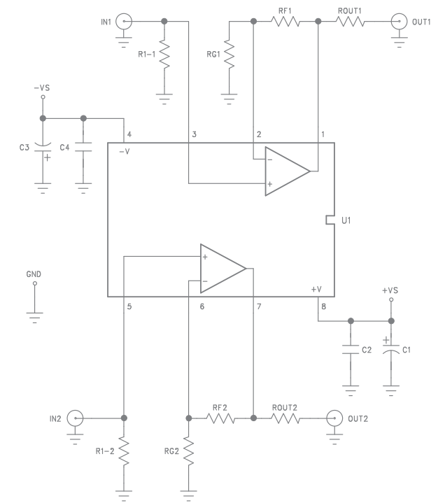
Figure 9. CEB006 Schematic
