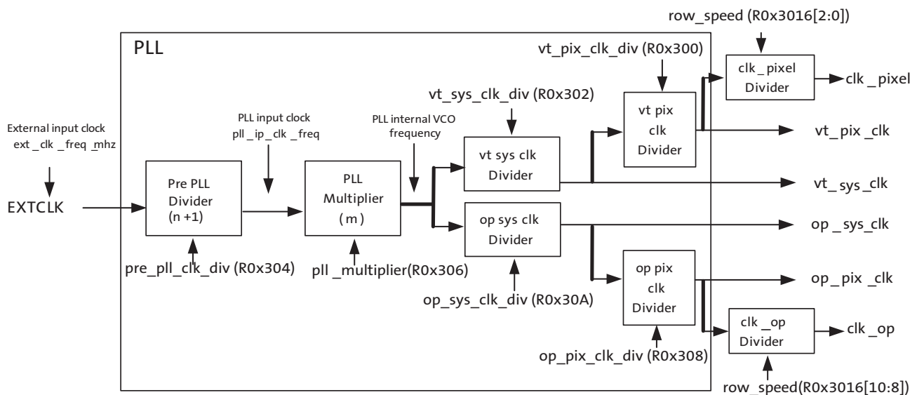
Figure 15: Clocking Configuration
