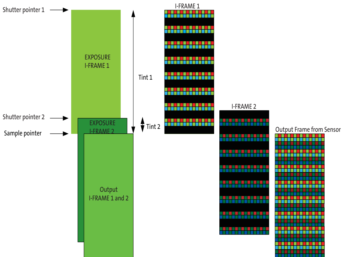
Figure 16: HDR Integration Time
