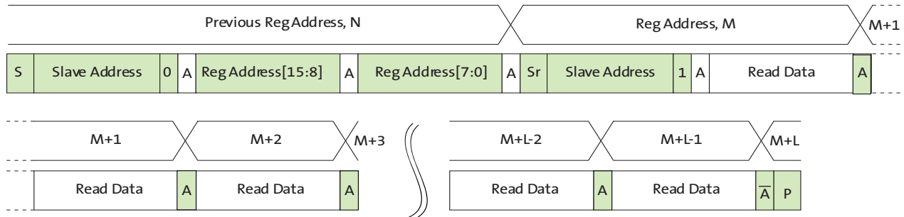
Figure 11: Sequential READ, Start from Random Location
