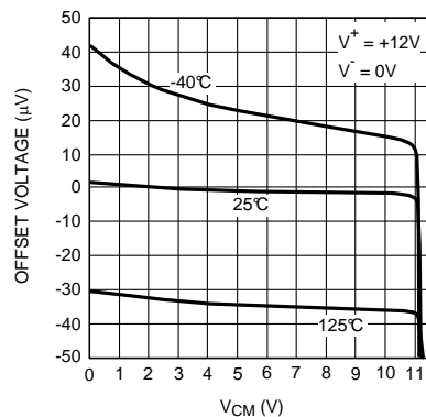
Figure 4. Offset Voltage vs V_{CM}
