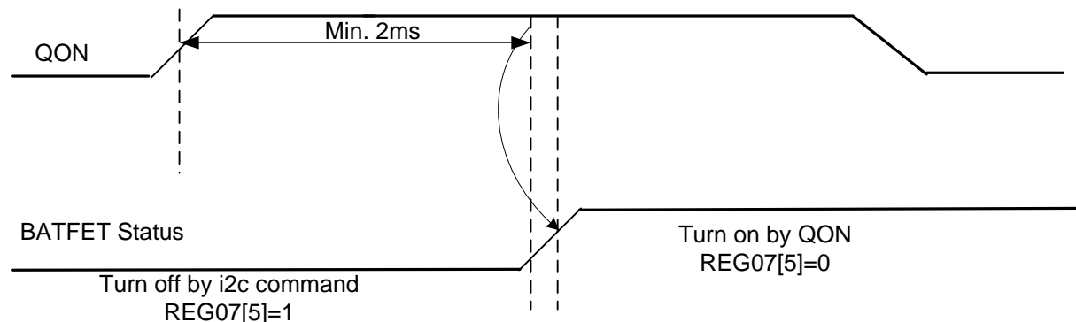
Figure 11. QON Timing
