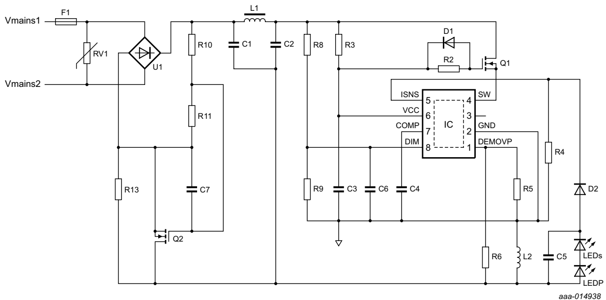
Fig 3. SSL5251T basic application diagram
