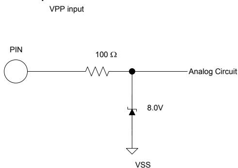
Figure 23 VPP programming pin
